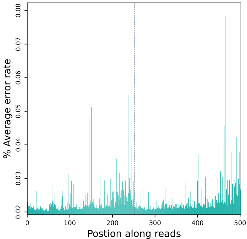
Error rate distribution along reads (R10117)
